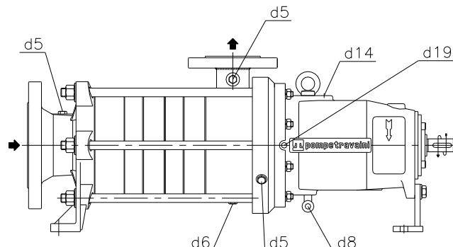
Pump series TBAK Standard connections and hook-ups
