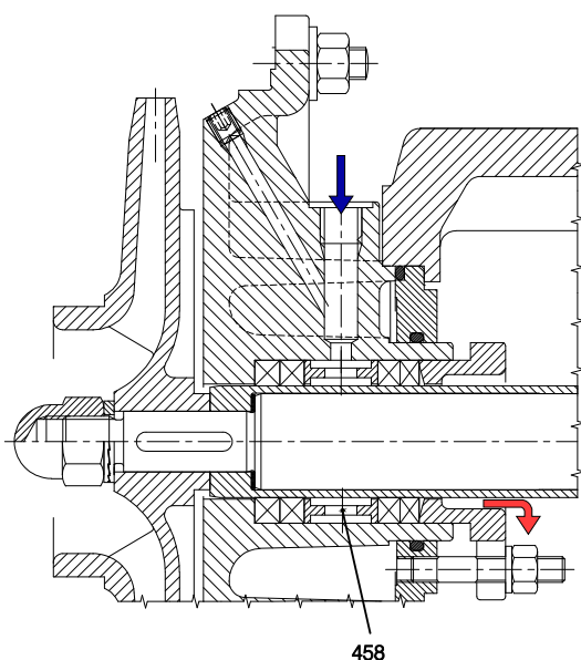
Fig.26c – PACKING WITH EXTERNAL FLUSHING (Plan 32)
