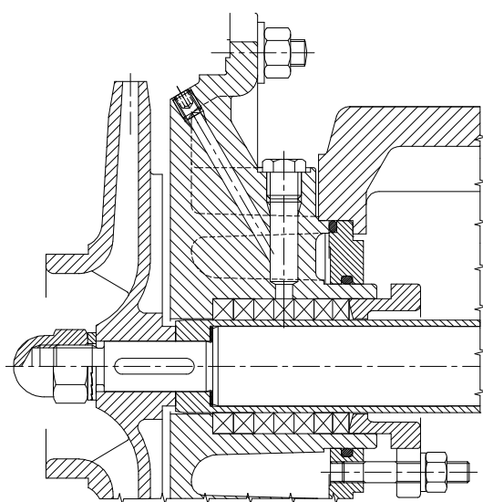
Fig.26c – PACKING WITH EXTERNAL FLUSHING (Plan 32)
