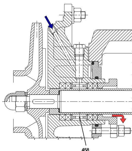
Fig.27d – PACKING WITH EXTERNAL FLUSHING AND WASH (Plan 62)
