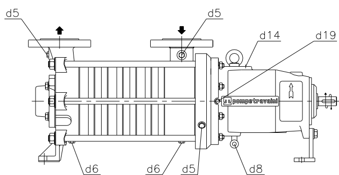
Pump series TBK Standard connections and hook-ups
