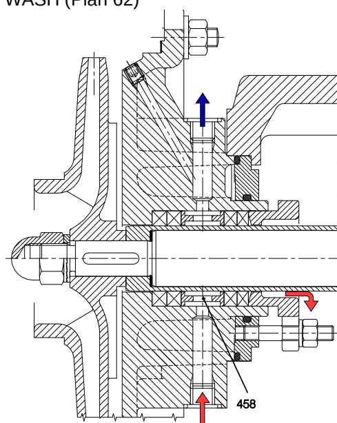
Fig.27d – PACKING WITH EXTERNAL FLUSHING AND WASH (Plan 62)
