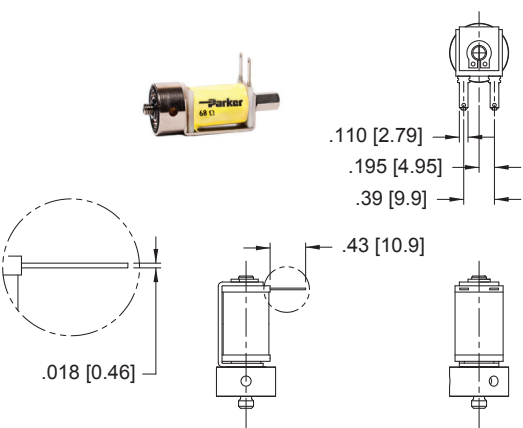
Coil Type: Quick Connect Spade (See Order Info "Q")
