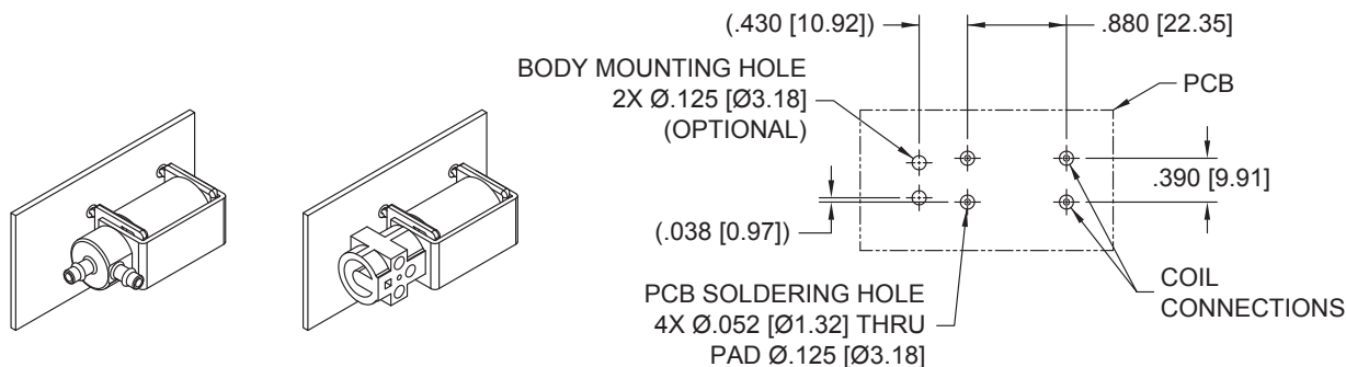
*PCB Pin Layout (Coil Type 4 PC Pin)
