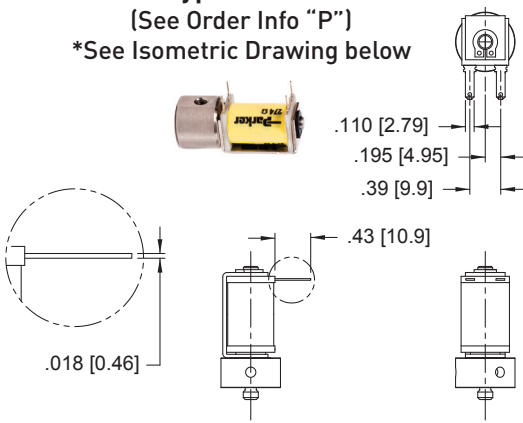
*4 PC PIN PCB Interface
