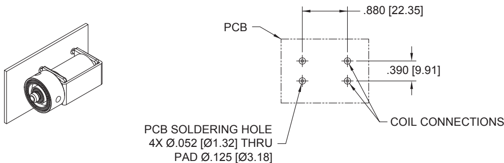
*4 PC PIN PCB Interface
